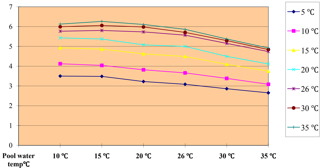
COP Curves at different air & water temperature
