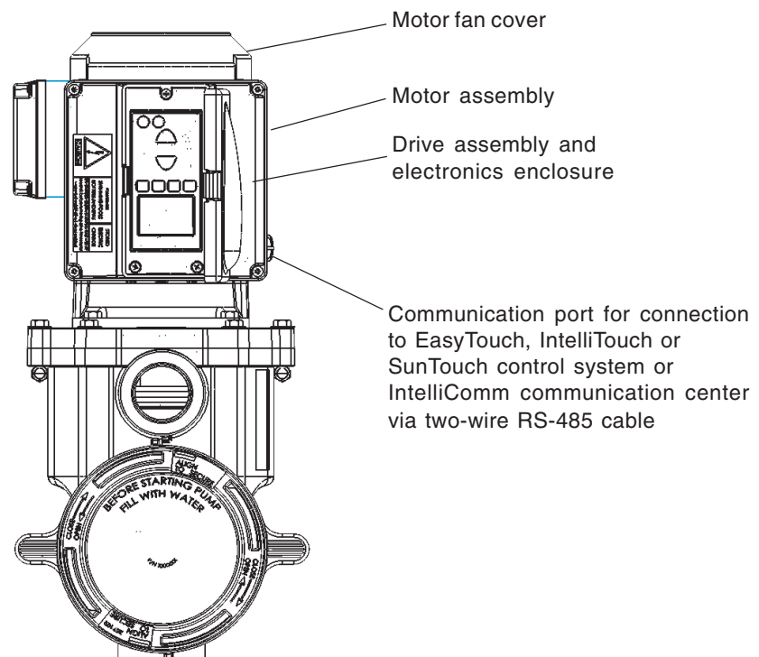
IntelliFlo VF (variable flow pump)
